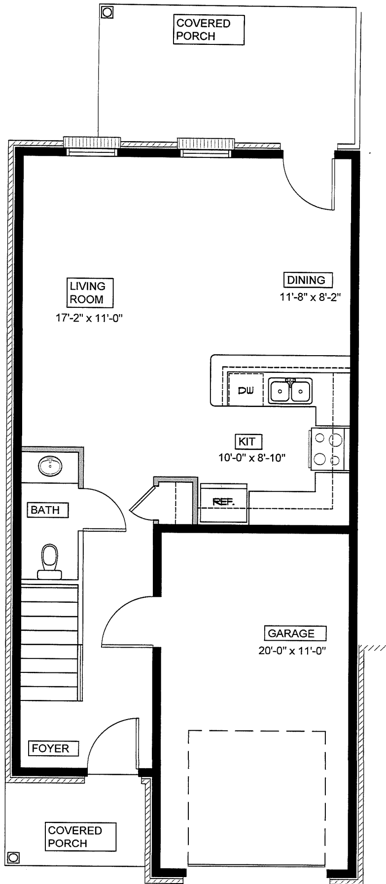
BLDG "A" and "C" and "X" "D" " FIRST FLOOR PLAN
