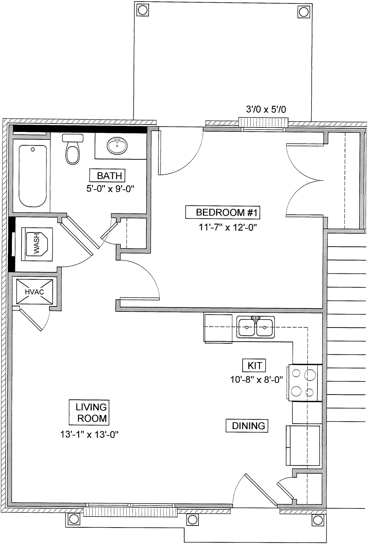
BLDG "E" FIRST FLOOR PLAN
